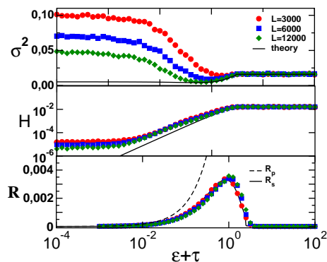
FIG. 4: Volatility (top), predictability (middle) and revenue (bottom) from speculators and producers for n_s = 60 and n_p = 1 . Markers are data obtained from numerical simulations of systems with different (effective) size L = PN_s with circles, squares and diamonds corresponding to L = 3000, 6000, 12000 respectively. Every data point represents an average over at least 1000 different strategy assignments. Simulations are run for 400P + 20N_s/(\varepsilon + \tau) steps, with measurements taken in the second half of this interval. Lines are the predictions of the analytical theory for the infinite system.
